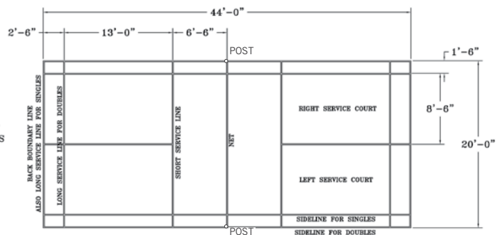
BADMINTON COURT LAYOUT
