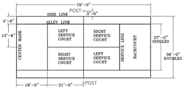
TENNIS COURT LAYOUT
