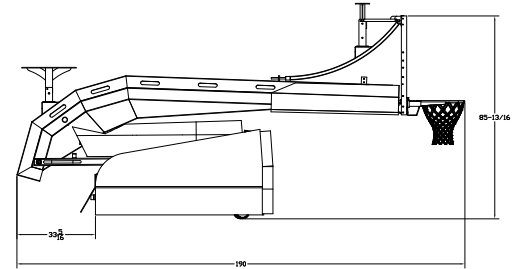
ARENA RENEGADE® BACKSTOP - 10' 8" Extension Footprint
