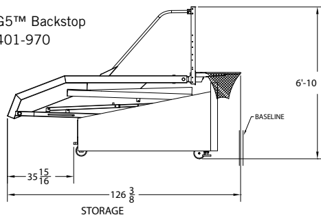
G5™ PORTABLE BACKSTOP storage dimensions: 126 3/8" long x 6' 10" high x 76" wide
