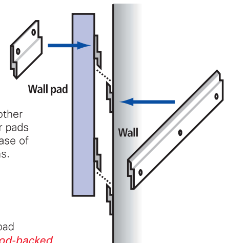
Z-Clip/Z-Bar systems: Side view
